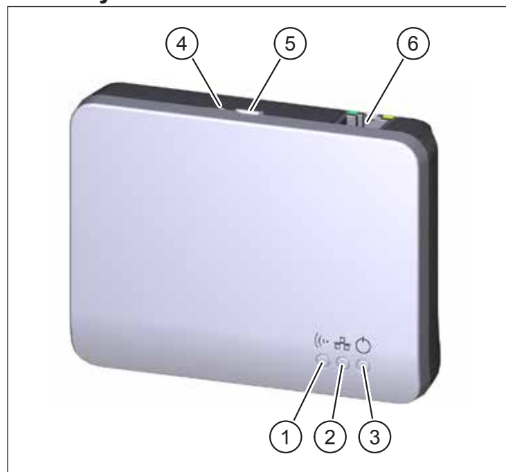
Obr. 1: Gateway M-WRG-GW
